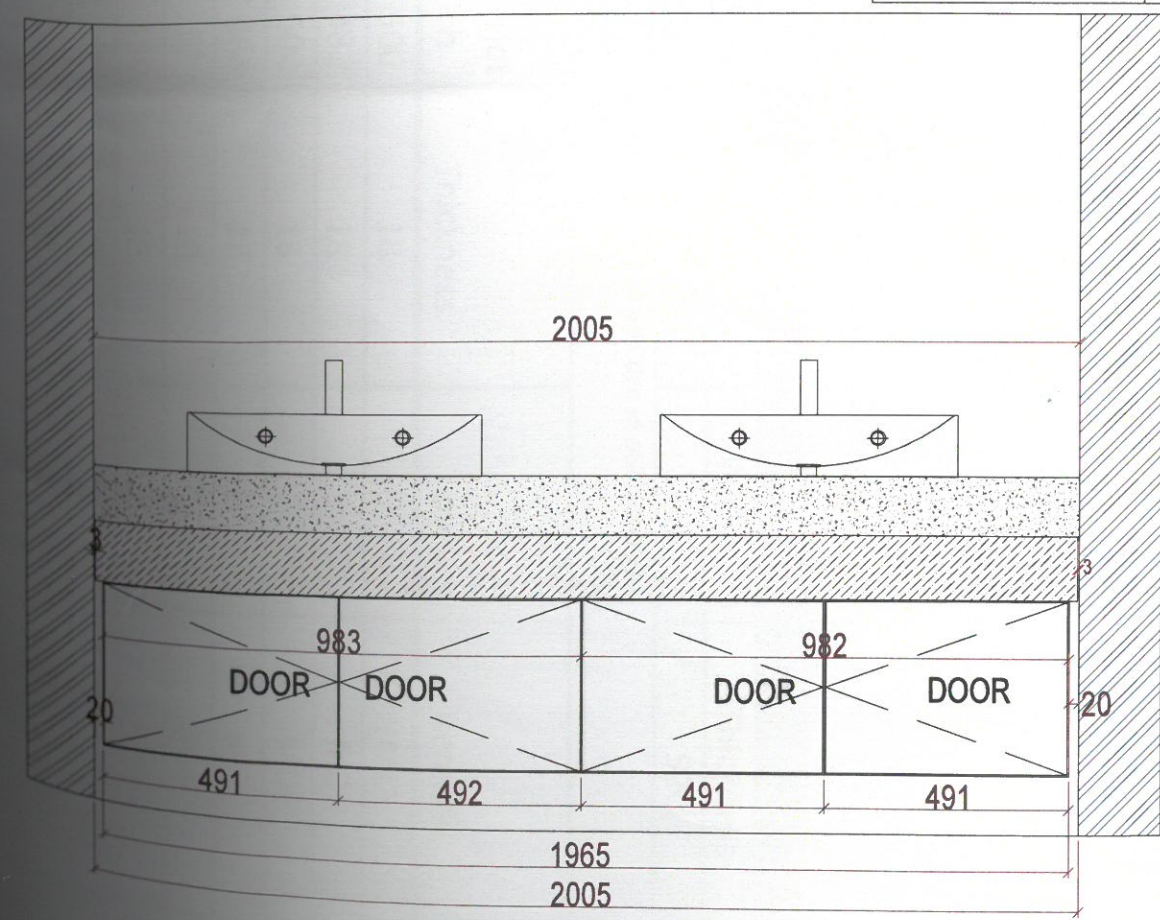
FRONT VIEW RAGHAV'S ROOM BATH -VANITY- 24TH FLOOR
